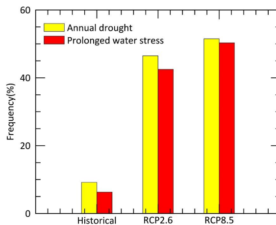
Figure 7. Compared to the historical data (1951–2005), the frequency of drought and prolonged water stress events will increase in Yunnan under the RCP2.6 and RCP8.5 projection scenarios (2006–2099).
