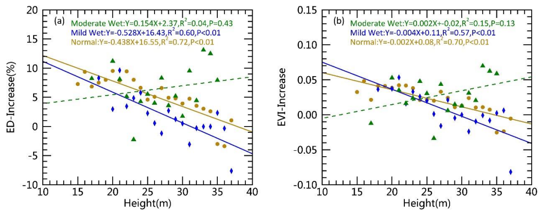
Figure 5. Linear regressions between the increase of EVI Deficit (ED) (from 2012 to 2014) and canopy height (a), and between enhanced vegetation index (EVI) (from 2012 to 2014) and canopy height (b) under three different water conditions (Normal: -0.5 < \text{SPEI} \leq 0.5 ; Mild Wet: 0.5 < \text{SPEI} \leq 1 ; Moderate Wet: 1 < \text{SPEI} \leq 1.5 ). The effects of canopy heights on forest recovery were no longer significant for the moderately wet condition.
