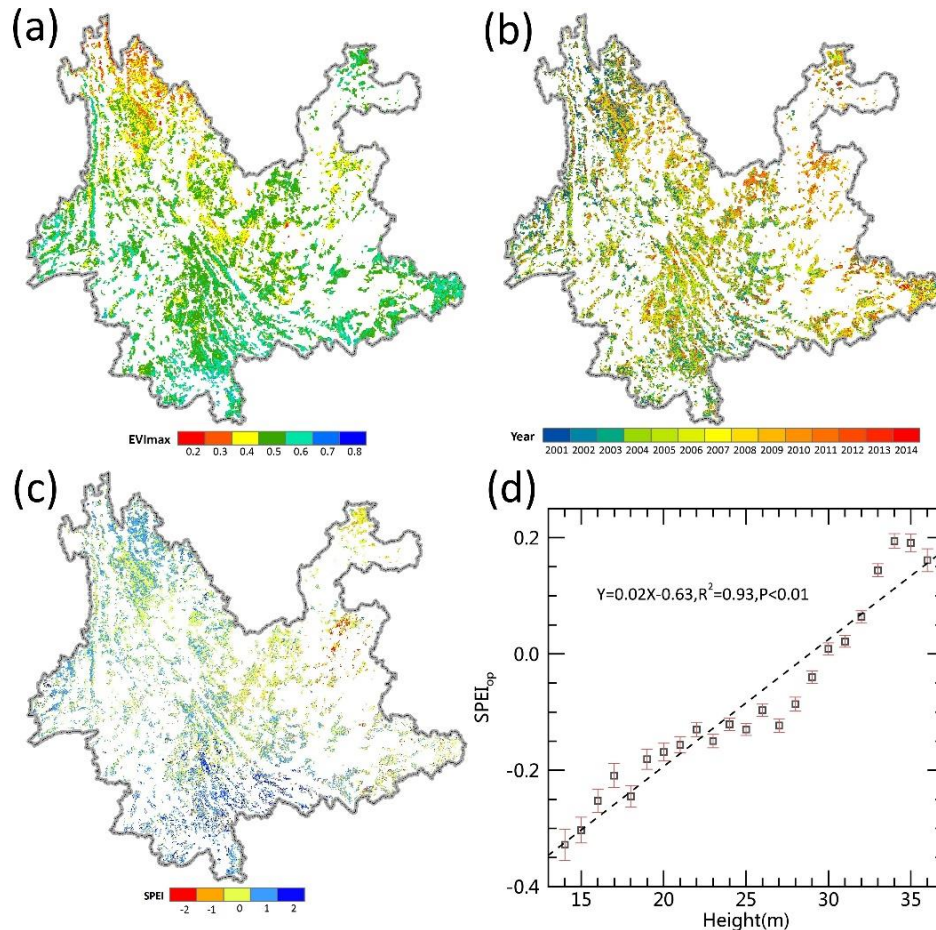
Figure 2. Water requirements of forest vary with canopy heights. (a) The maximum enhanced vegetation index (EVI) of forests in Yunnan during 2001–2014; (b) The occurrence time of the maximum EVI in (a); (c) The standardized precipitation evapotranspiration index (SPEI) value at the occurrence time of the maximum EVI ( SPEI_{op} , which represents the optimal water availability for maximum growth potential); (d) Regression of mean SPEI_{op} against forest canopy height (mean SPEI_{op} were calculated for pixels with the same canopy heights). The white regions in (a–c) represent nonforest areas.
