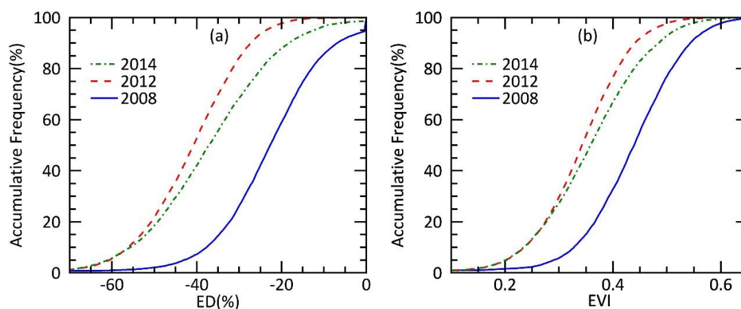
Figure 4. EVI Deficit (ED) (a) and enhanced vegetation index (EVI) (b) in the recovery areas, affected by drought during 2009–2013 and with improved water condition in 2014, before (blue, 2008), during (red, 2012), and after drought stress (green, 2014).
