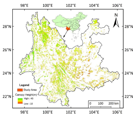
Figure 1. The distribution and canopy heights of forested area in Yunnan Province, southwest China, at a resolution of 1 km [21]. The white region represents the nonforest area.
