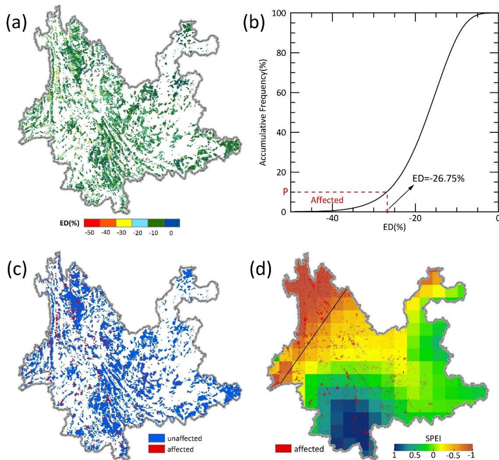
Figure 3. The determination of forest recovery area: (a) Average ED (EVI Deficit (%); EVI: enhanced vegetation index) of forested areas during the drought event of 2009–2012 in Yunnan Province. (b) The top 10% area with the most negative ED ( < -26.75\% ) was selected as the drought-affected area for this study. (c) Forested area in Yunnan was further divided into two regions: affected ( ED < -26.75\% , red) vs. unaffected ( ED \geq -26.75\% , blue). (d) Standardized precipitation evapotranspiration index (SPEI) of Yunnan Province in 2014. Forest areas affected by the prolonged drought during 2009–2013 ( ED < -26.75\% , red spots in (c,d)) with water condition improved in 2014 ( SPEI > -0.5 , red spots below the black line in (d)) were defined as the potential recovery area of the forest. The white regions in (a,b) represent nonforest land.
