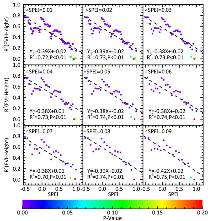
Figure 6. The relationship between forest recovery and canopy height under various water availability. The x -axis (SPEI, standardized precipitation evapotranspiration index) represents water availability, and the y -axis indicates the determination coefficients ( R^2 ) of the regression equation between the increase of enhanced vegetation index (EVI) from 2012 to 2014 and canopy height. The color-bar indicates the significance of the regression equation. With improved water availability, the relationship between forest recovery and canopy height weakened, suggesting that height is an important factor affecting forest recovery, but its effect depends on water availability and will disappear with sufficient water. The nine panels (with varying delta SPEI) showed a consistent pattern.
