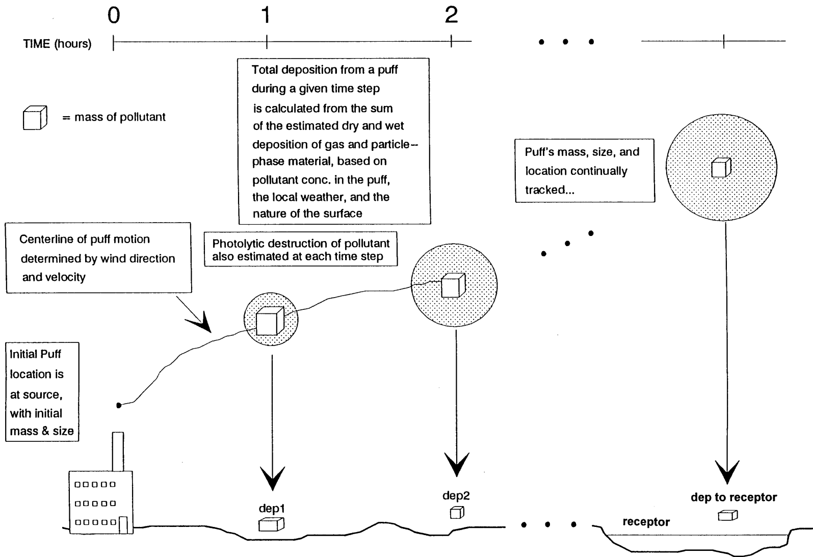
Figure 1 HYSPLIT Air Transport and Deposition Model
