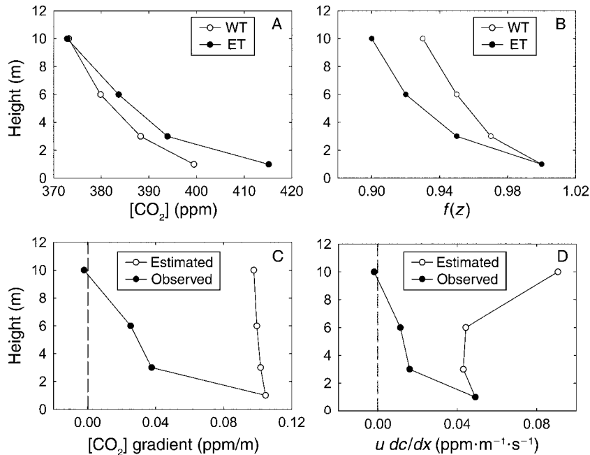
FIG. 3. (A) \text{CO}_2 profiles at ET and WT; (B) relative distribution functions of \text{CO}_2 at ET and WT; (C) horizontal \text{CO}_2 gradients; and (D) horizontal advection u \, dc/dx . The “estimated” horizontal \text{CO}_2 gradients (open circles in C) and u \, dc/dx (open circles in D) were derived based on the relative distribution function of \text{CO}_2 at WT and \text{CO}_2 concentration at 1 m measured at ET. The u_* for this case is 0.36 m/s. Data are from 05:30 hours Mountain Standard Time on 24 June 2002. Variables are: f , frequency; z , height above the ground (in meters); u , horizontal wind speed (in m/s); u_* , surface friction velocity (m/s); c , concentration of \text{CO}_2 (ppm \text{CO}_2 per million parts of air).
