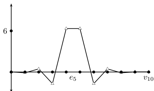
FIGURE 4. Coefficients of v_i appearing in \star e_5 , for n=10
